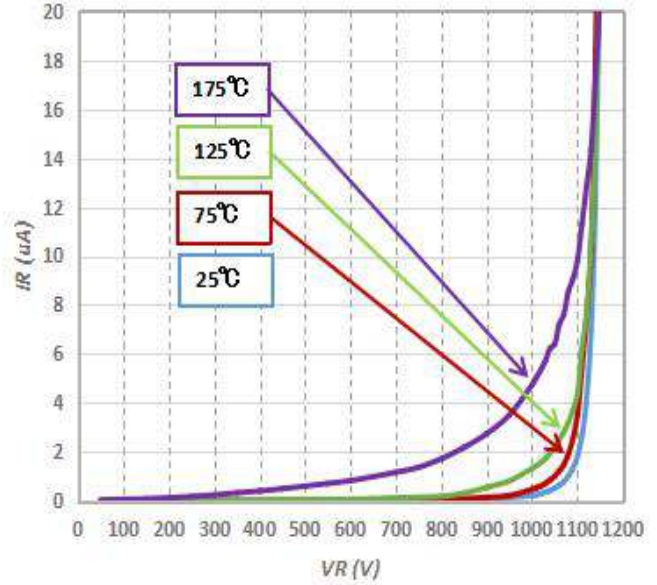
Fig.2-Typical Reverse Characteristics
