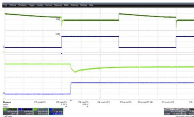
Figure 22 – Transient Response Min = 4.08 V, Max = 5.33 V. 115 VAC, 0-2 A Load Step. Upper: I_{LOAD} , 1 A / div. Lower: V_{OUT} , 500 mV, 50 ms / div.
