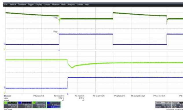
Figure 24 – Transient Response Min = 4.18 V, Max = 5.34 V. 265 VAC, 0-2 A Load Step. Upper: I_{LOAD} , 1 A / div. Lower: V_{OUT} , 500 mV, 50 ms / div.
