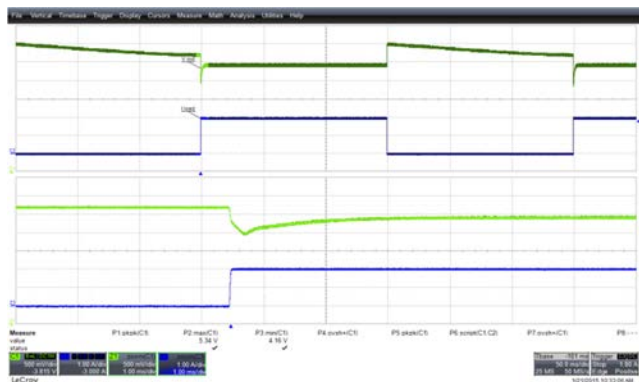
Figure 23 – Transient Response Min = 4.16 V, Max = 5.34 V. 230 VAC, 0-2 A Load Step. Upper: I_{LOAD} , 1 A / div. Lower: V_{OUT} , 500 mV, 50 ms / div.
