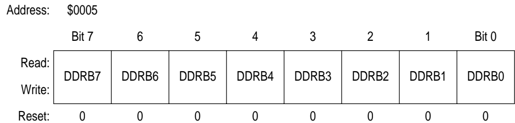
Figure 17-7. Data Direction Register B (DDRB)
