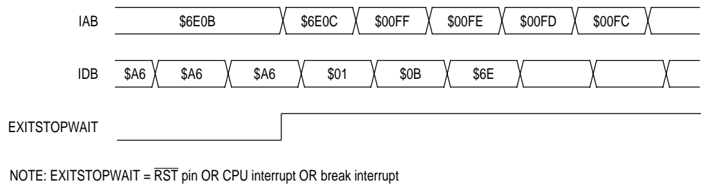
Figure 9-15. Wait Recovery from Interrupt or Break
