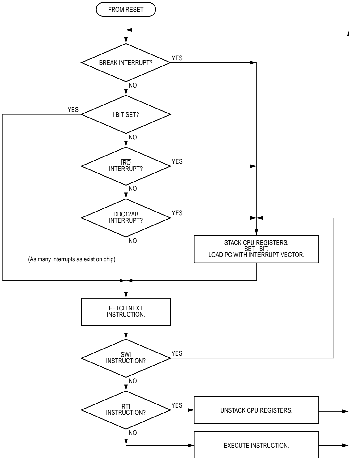
Figure 9-10. Interrupt Processing
