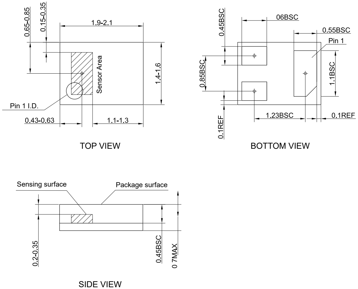
Figure 19. Package outline of LGA3L (unit: mm)
