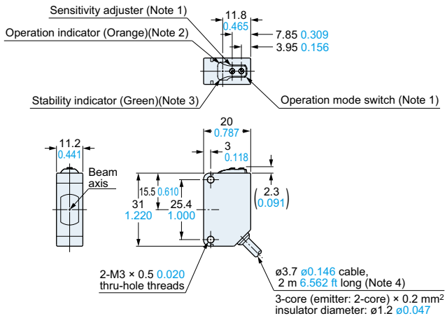
CX-41□ Sensor
