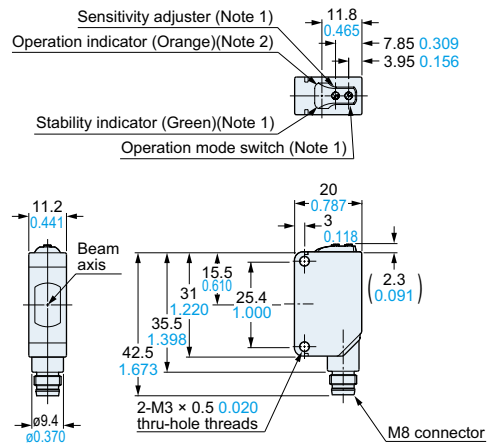
CX-41□-Z Sensor
