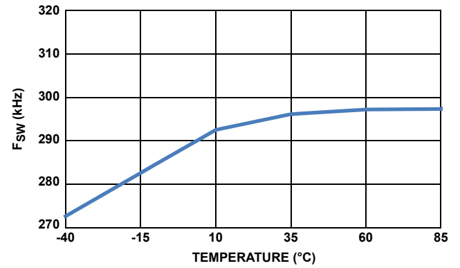
FIGURE 14. f_{SW} vs TEMPERATURE
