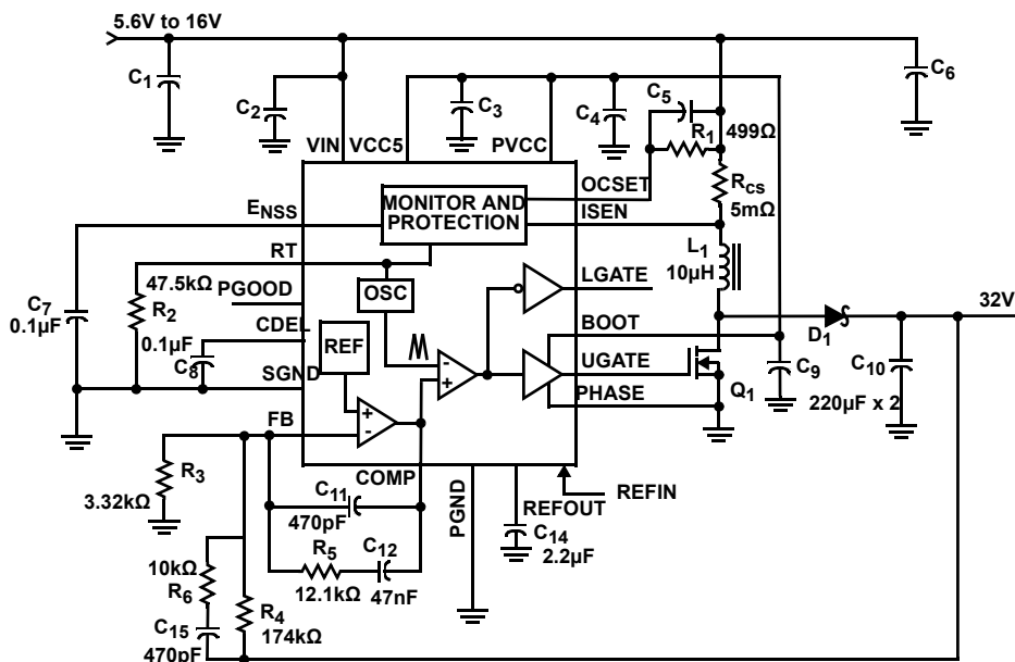
FIGURE 1. BOOST CONVERTER
