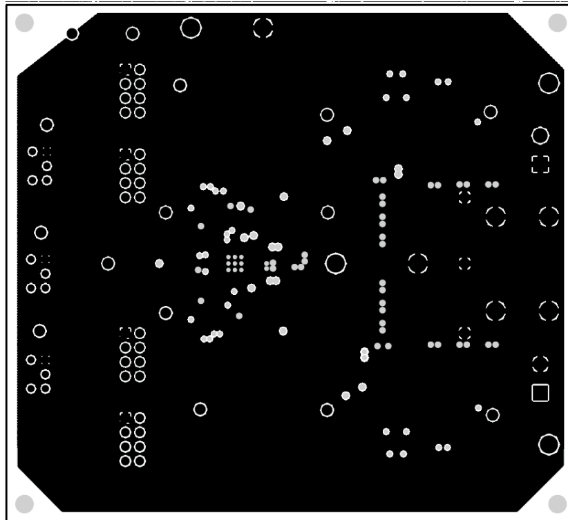
Figure 7-2. Inner Layer 1
