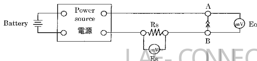
Fig.7 Block diagram of measuring equipment of low-level contact resistance
