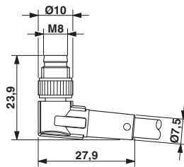
Plug M8 x 1, angled, shielded
