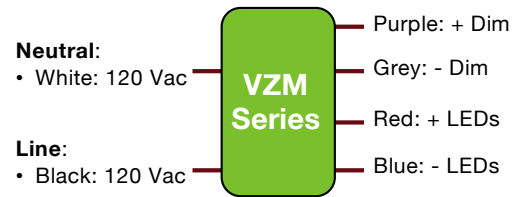
Wiring Diagram
