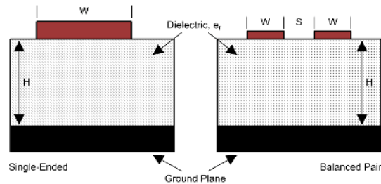
Figure 15. Microstrip Topology
