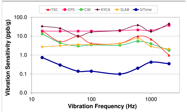
Figure 16. Vibration Robustness [5]
