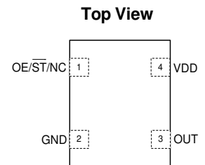
Figure 1. Pin Assignments
