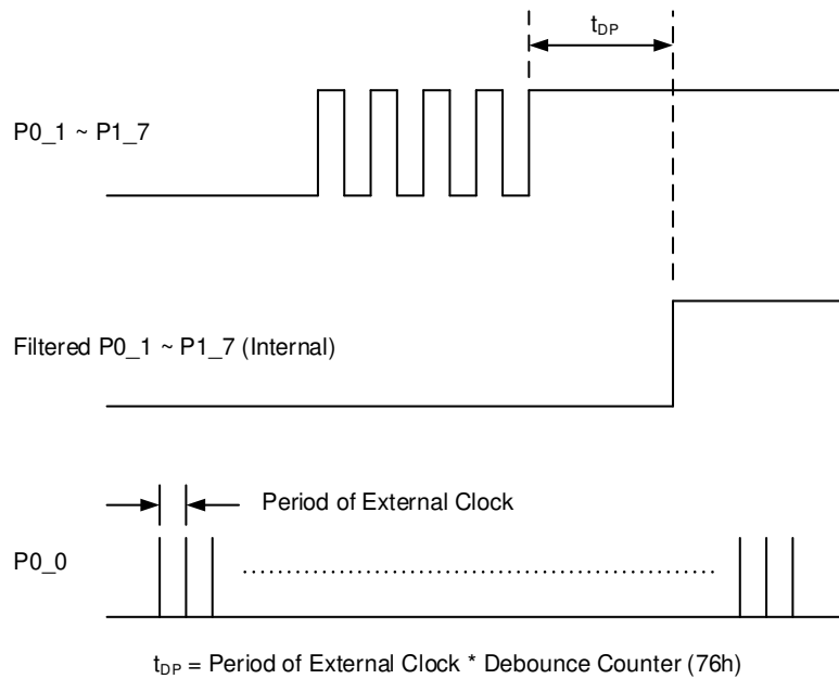
Figure 6. Debounce Timing
