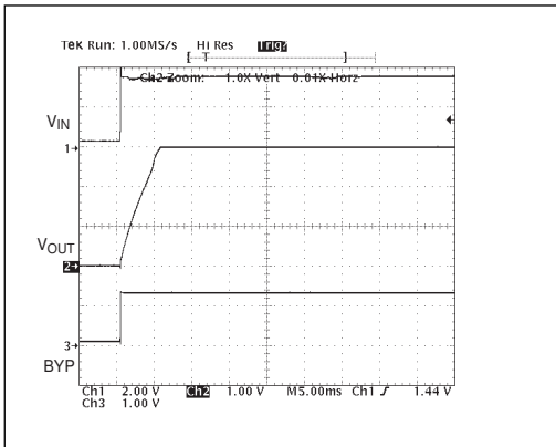
Fast V_{IN} , C_{OUT}=1000\mu\text{F} , I_O=500\text{mA}
