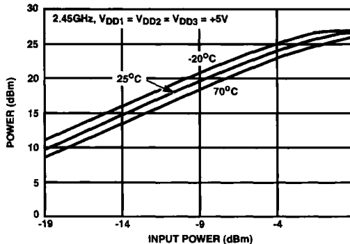
FIGURE 8. POWER OUTPUT
