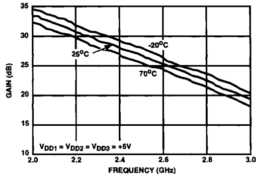
FIGURE 7. LINEAR GAIN
