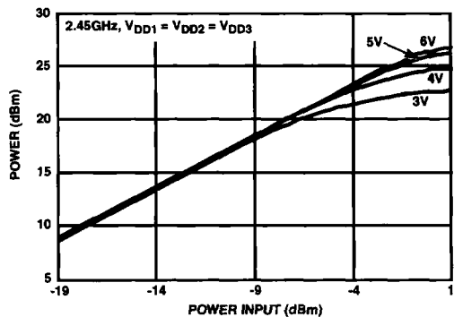
FIGURE 4. POWER OUTPUT
