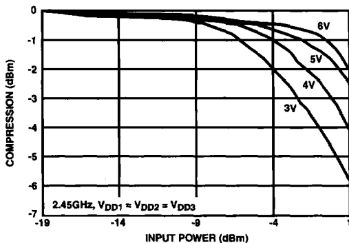
FIGURE 6. GAIN COMPRESSION
