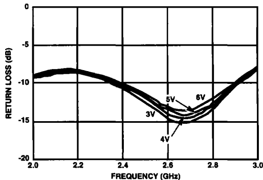
FIGURE 3. OUTPUT MATCH
