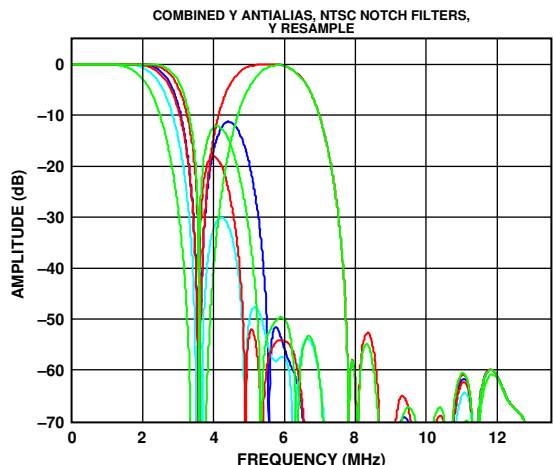
Figure 15. NTSC Notch Filter Response
