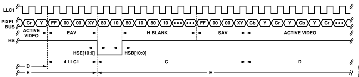
Figure 20. HS Timing
