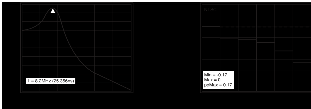
Figure 5. Group Delay vs. Frequency
