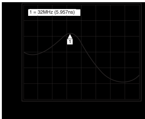
Figure 9. Group Delay vs. Frequency
