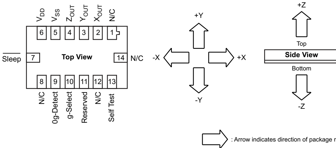
Figure 2. Pin-Out and Polarity for MMA73x0L
