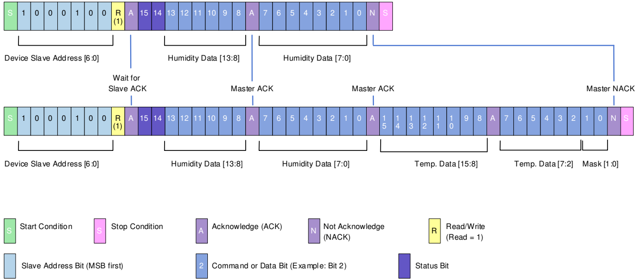
Figure 13. Data Fetch
