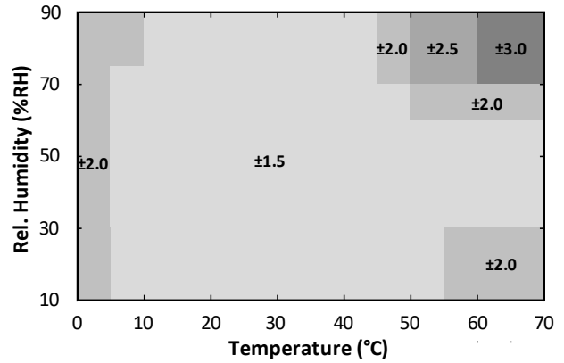
Figure 5. HS3101-MCx RH Accuracy over Temperature
