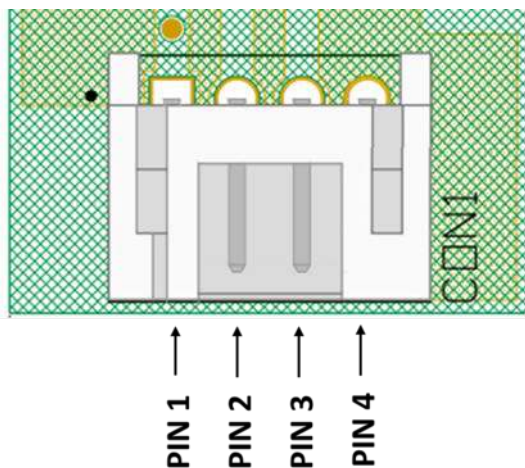
Figure 1. Pin Assignments
