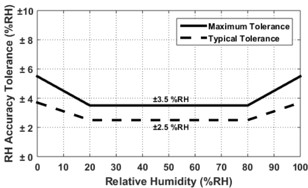
Figure 6. HS3103-MCx RH Accuracy Tolerance at 25°C
