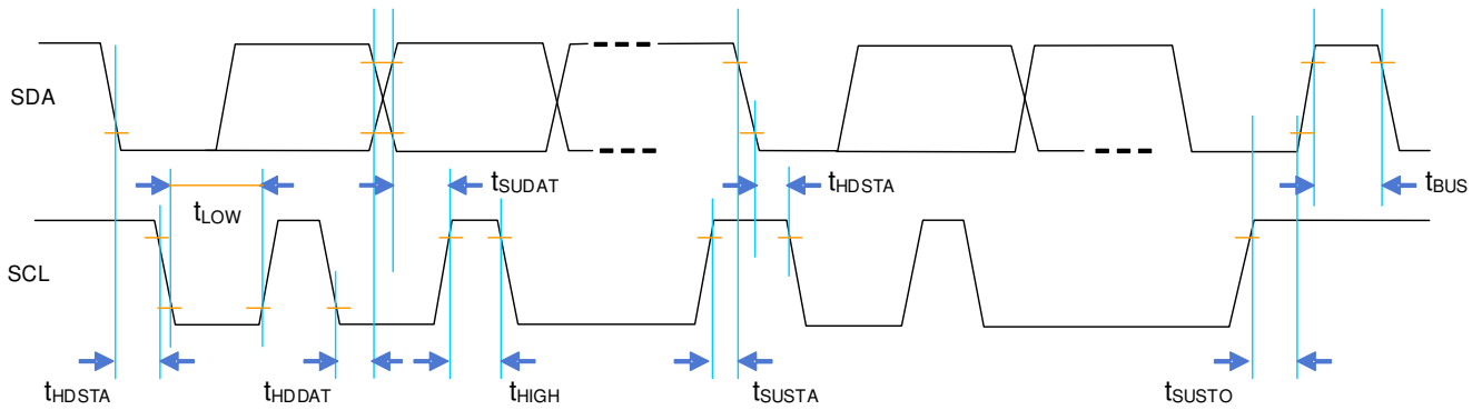
Figure 10. Timing Diagram
