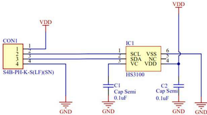
Figure 16. HS310x-MCx Application Circuit
