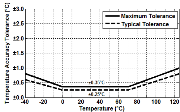
Figure 9. HS3103-MCx Temperature Sensor Accuracy Tolerance
