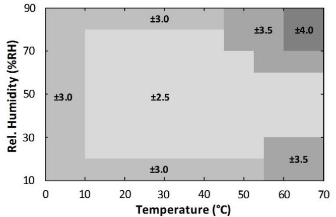
Figure 7. HS3103-MCx RH Accuracy over Temperature
