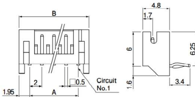
Figure 2. Pin Connector
