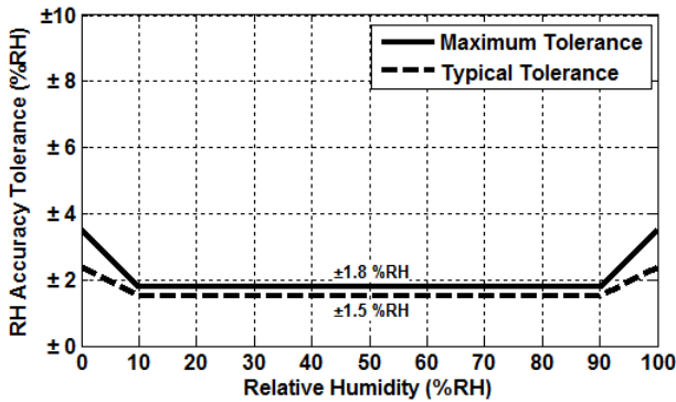
Figure 4. HS3101-MCx RH Accuracy Tolerance at 25°C
