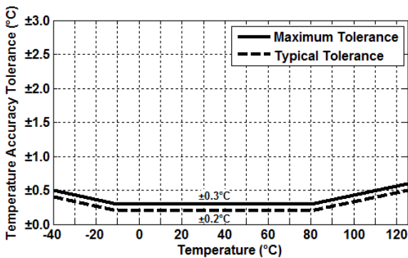
Figure 8. HS3101-MCx Temperature Sensor Accuracy Tolerance
