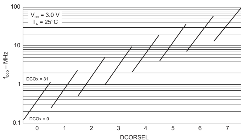
Figure 5-2. Typical DCO Frequency
