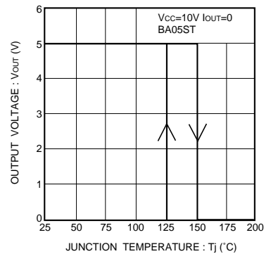
Fig.9 Thermal cutoff circuit characteristics
