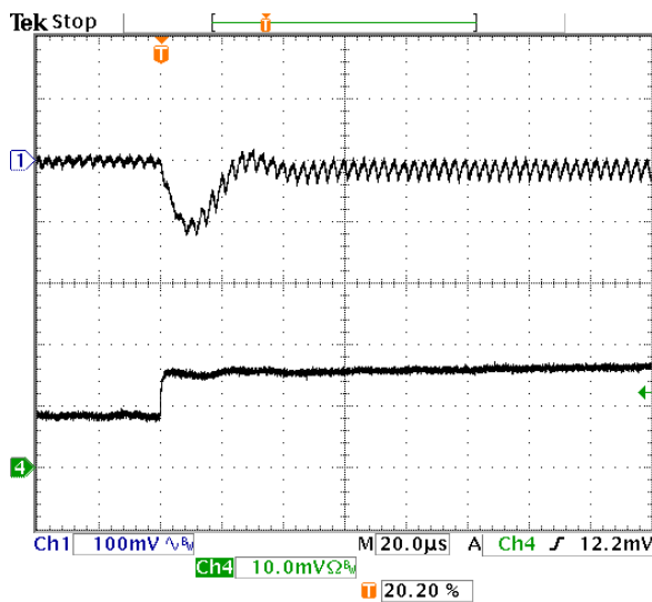
Fig-1.5V-6: Output voltage response for V_{out}=1.5V to positive load current step-change from 4A to 8A with slew rate of 5A/\mu s at V_{in}=5.0V . C_o=47\mu F \times 2 ceramic + 1\mu F ceramic. Top trace: output voltage (100mV/div.) Bottom trace: load current (5A/div.) Time scale: 20µs/div.
