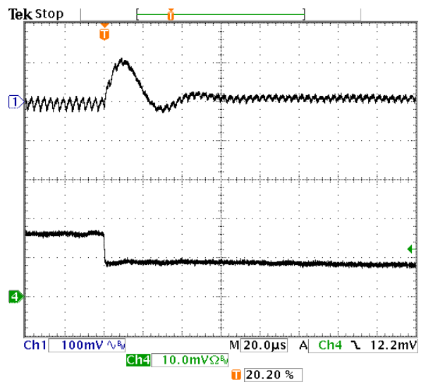
Fig-1.5V-7: Output voltage response for V_{out}=1.5V to positive load current step-change from 8A to 4A with slew rate of -5A/\mu s at V_{in}=5.0V . C_o=47\mu F \times 2 ceramic + 1\mu F ceramic. Top trace: output voltage (100mV/div.) Bottom trace: load current (5A/div.) Time scale: 20µs/div.
