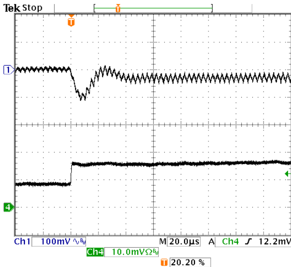
Fig-2.5V-6: Output voltage response for V_{out}=2.5V to positive load current step-change from 4A to 8A with slew rate of 5A/\mu s at V_{in}=5.0V . C_o=47\mu F \times 2 ceramic + 1\mu F ceramic.
