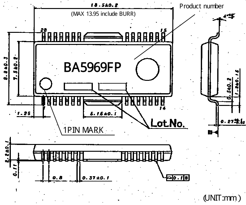
fig.1 PACKAGE OUTLINES
