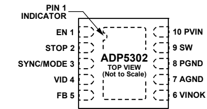
Figure 3. Pin Configuration
