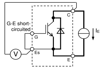
V_{EC} characteristics test circuit
