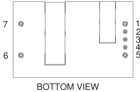
Figure 53. 0RQB-50Y12L/0 Pins
