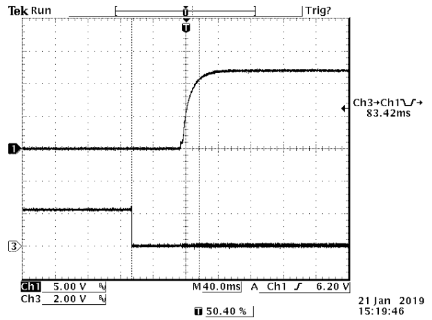
Figure 33. Startup from on/off Ch1: Vo Ch3: on/off Test Condition: Vin=110V, Io=4.2A, Vo=12V with Cext=1200uF
