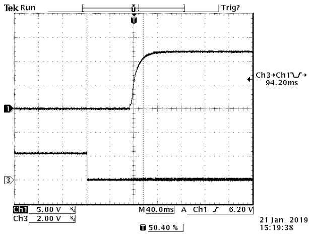
Figure 32. Startup from on/off Ch1: Vo Ch3: on/off Test Condition: Vin=48V, Io=4.2A, Vo=12V with Cext=1200uF
