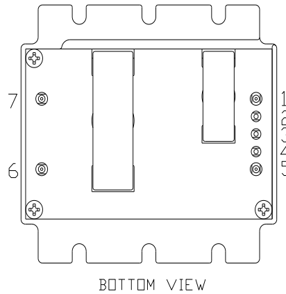
Figure 57. 0RQB-50Y12E/F Pins
