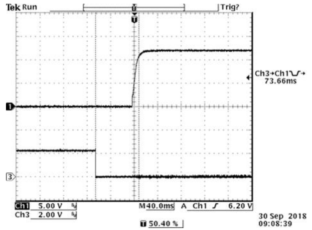
Figure 31. Startup from on/off Ch1: Vo Ch3: on/off Test Condition: Vin=110V, Io=4.2A, Vo=12V with Cext=200uF
