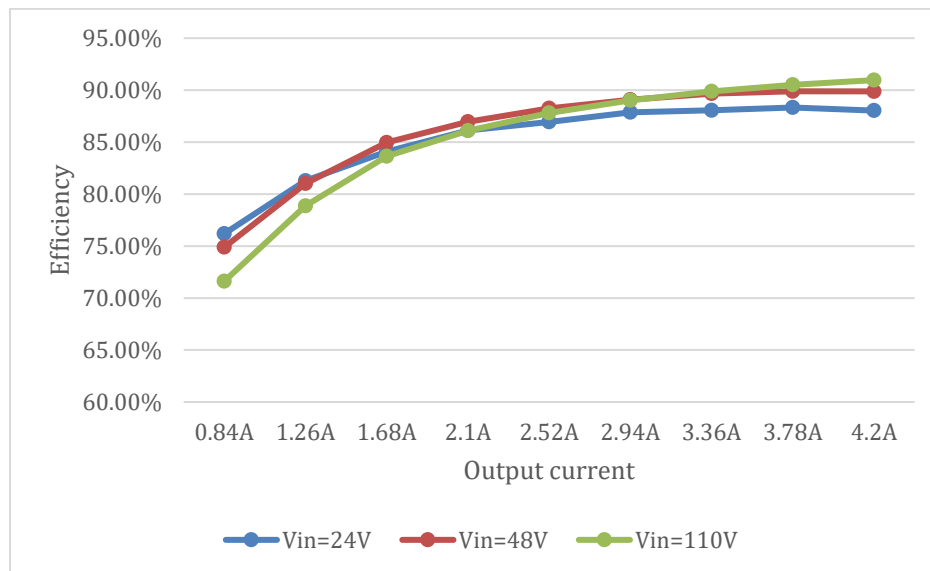
Figure 1. Efficiency data
