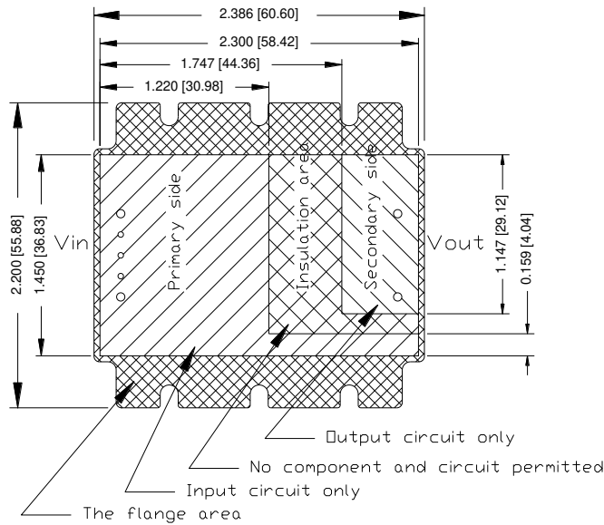
Figure 58. 0RQB-50Y12E/F Recommended pad layout-1
