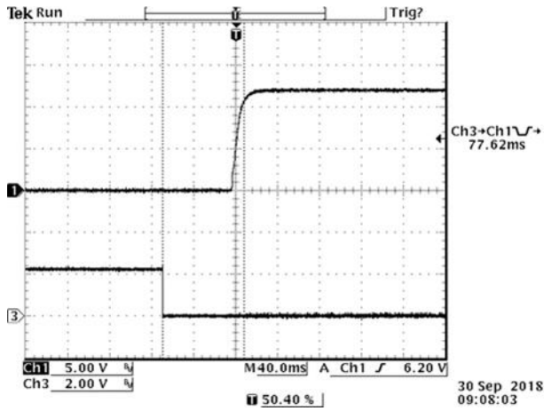
Figure 30. Startup from on/off Ch1: Vo Ch3: on/off Test Condition: Vin=48V, Io=4.2A, Vo=12V with Cext=200uF
