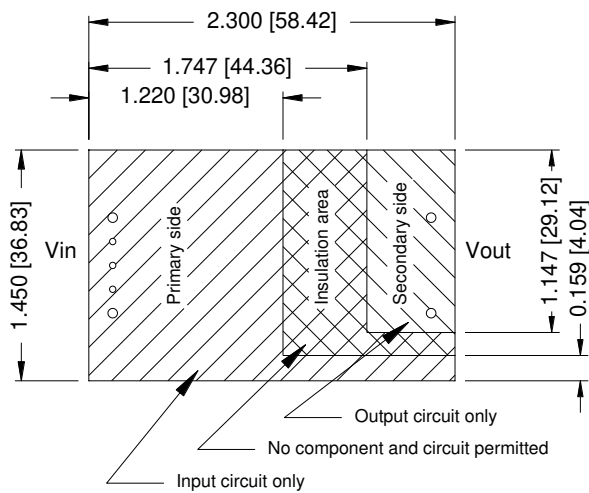
Figure 54. 0RQB-50Y12L/0 Recommended pad layout-1
