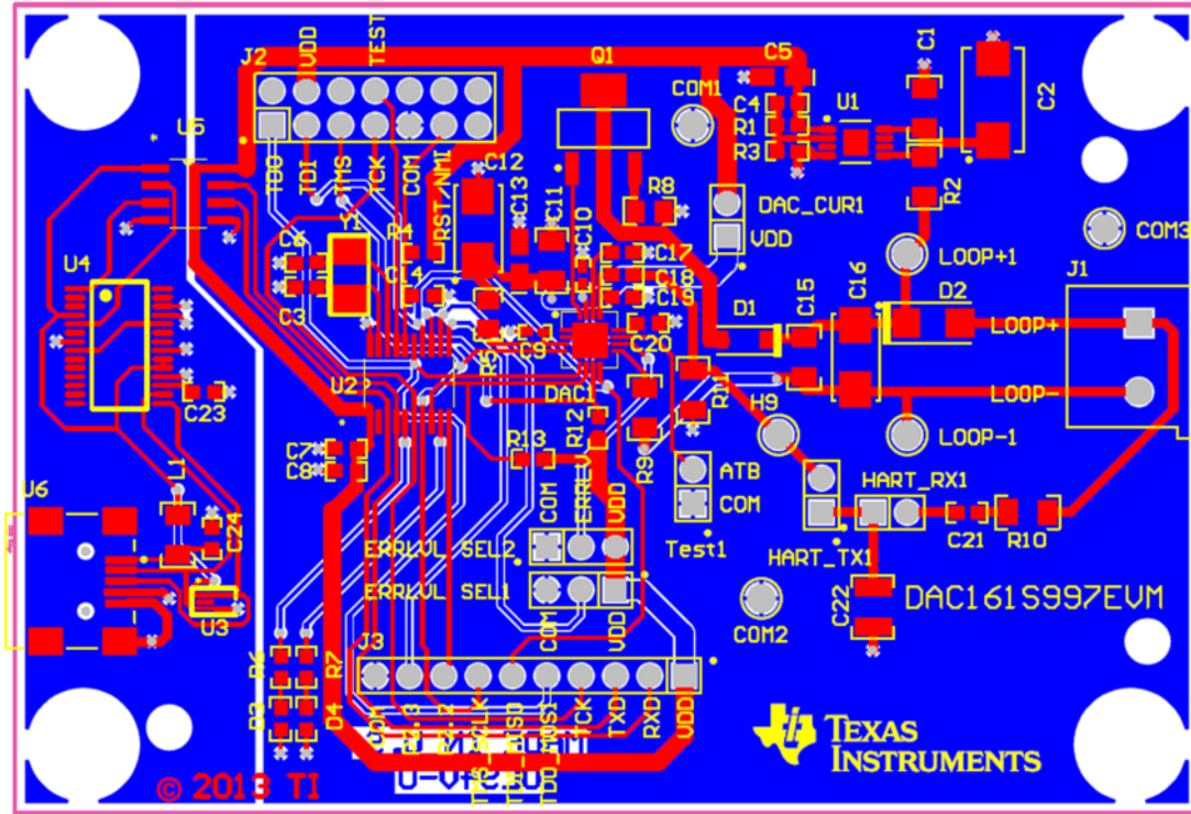
Figure 10. Top Assembly Layer
