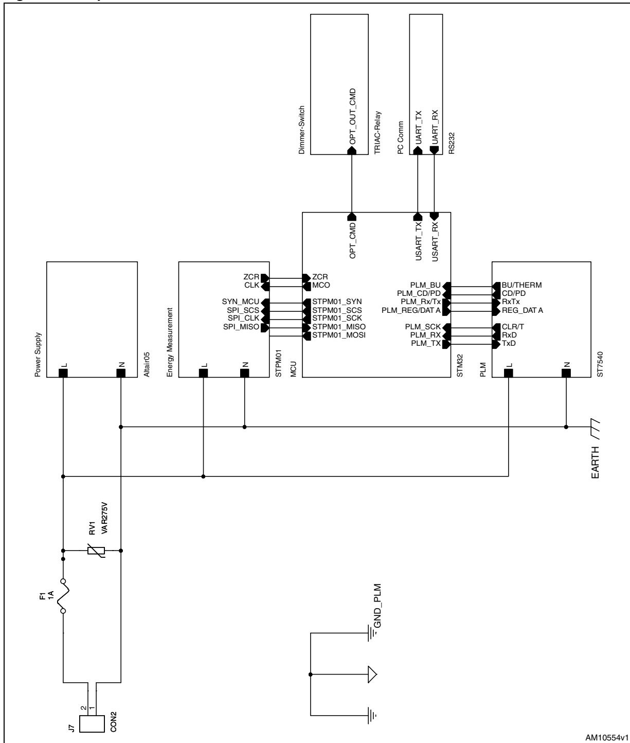
Figure 1. Top-level schematic
