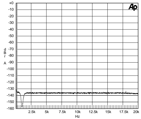
Figure 17. -20 dBFS FFT
