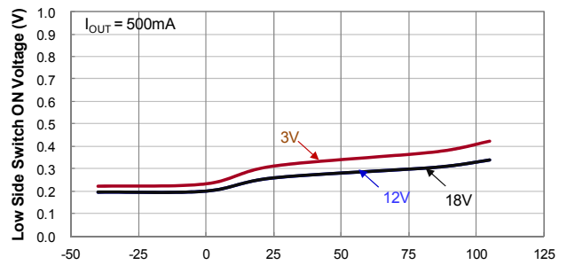
Low Side Switch ON Voltage V_{OL} vs. Temperature
