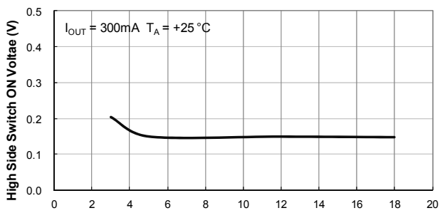
High Side Switch ON Voltage ( V_{DD} - V_{OH} ) vs. Supply Voltage
