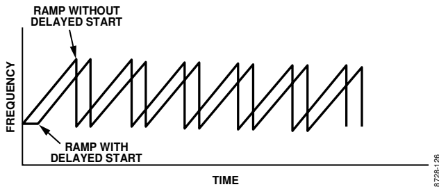
Figure 38. Delayed Start of Sawtooth Ramp
