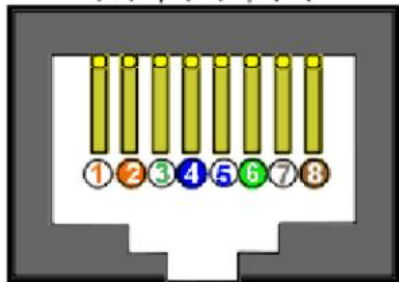
RJ-45 JACK
