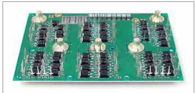
(48) FETs (9) Low profile capacitors (5) Low profile bus bars Total Weight 0.82 lbs (370.6 g)
