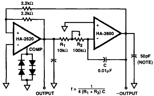
FIGURE 2. FUNCTION GENERATOR
