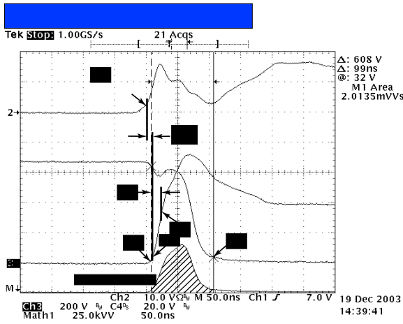
Figure 18, Turn-on Switching Waveforms and Definitions
