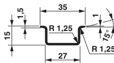
Dimensional drawing
