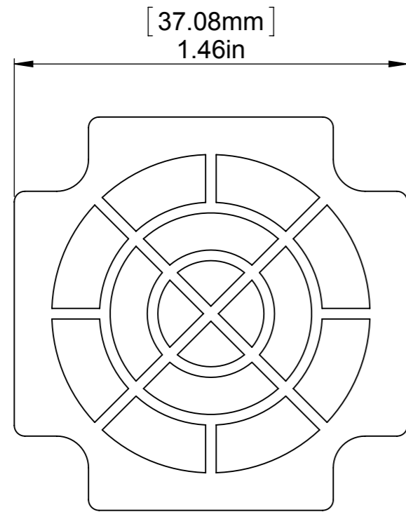
Retainer
