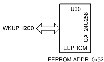
Figure 9. Board ID EEPROM
