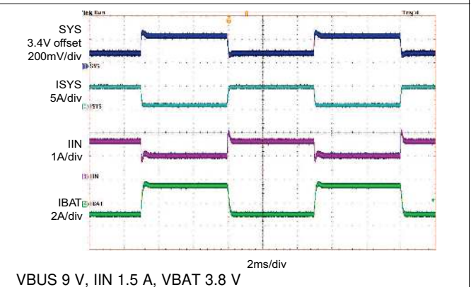
Figure 38. Charge Disable
