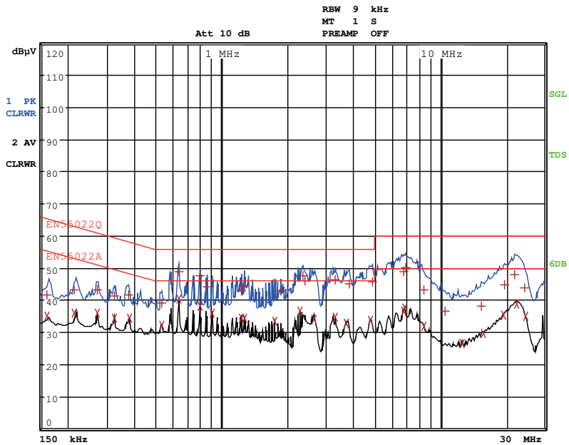
230Vac, 50Hz, Maximum Load, L Line, Output GND connects to Earth, EN5022 Limits
