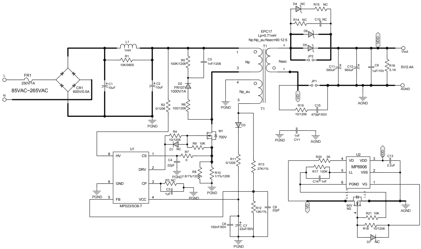
Figure 1—Schematic
