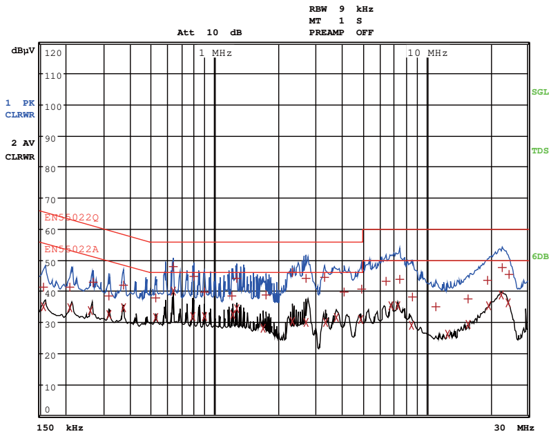
230Vac, 50Hz, Maximum Load, N Line, Output GND connects to Earth, EN5022 Limits
