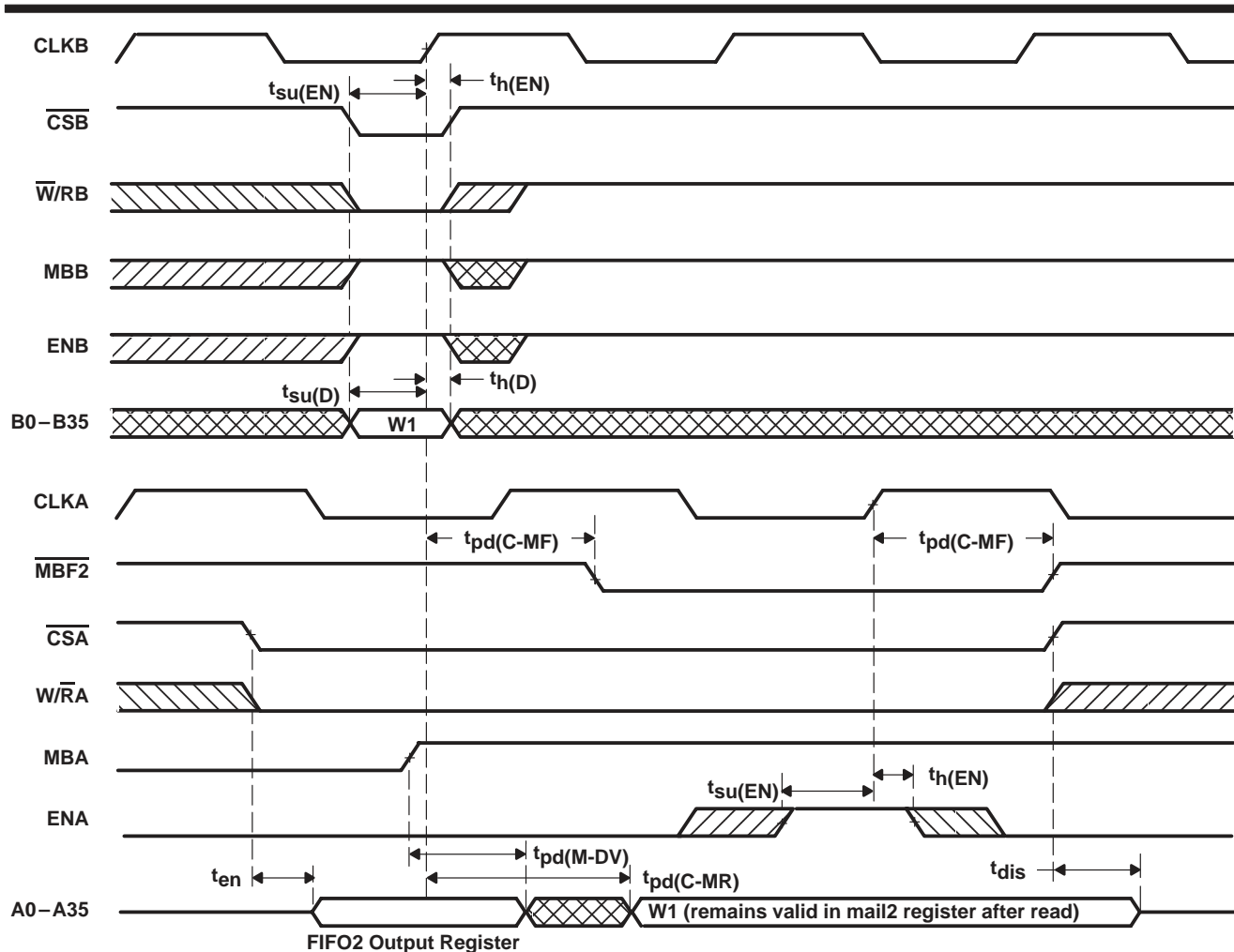
Figure 16. Timing for Mail2 Register and \overline{MBF2} Flag
