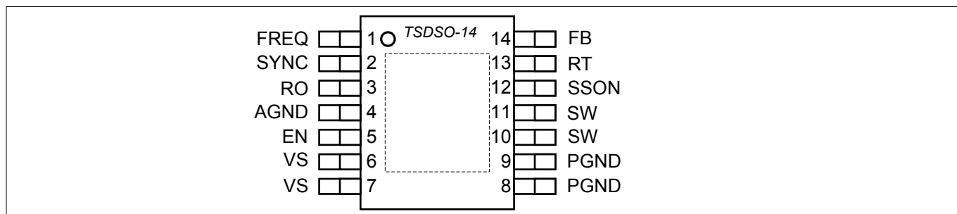
Figure 2 Pin configuration
