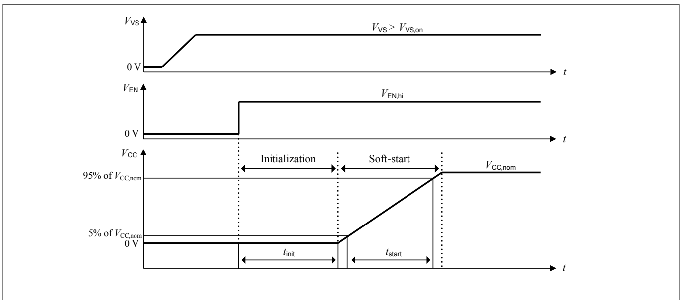
Figure 6 Typical startup procedure
