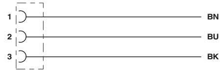
Contact assignment of the DEUTSCH DT06-3S
