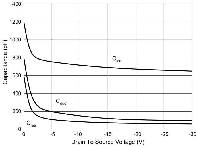
Fig. 12 - Capacitance Characteristics
