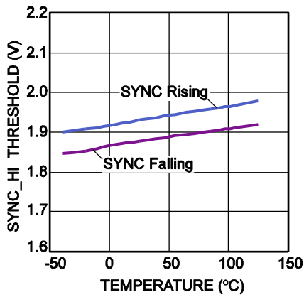
Sync_Hi
