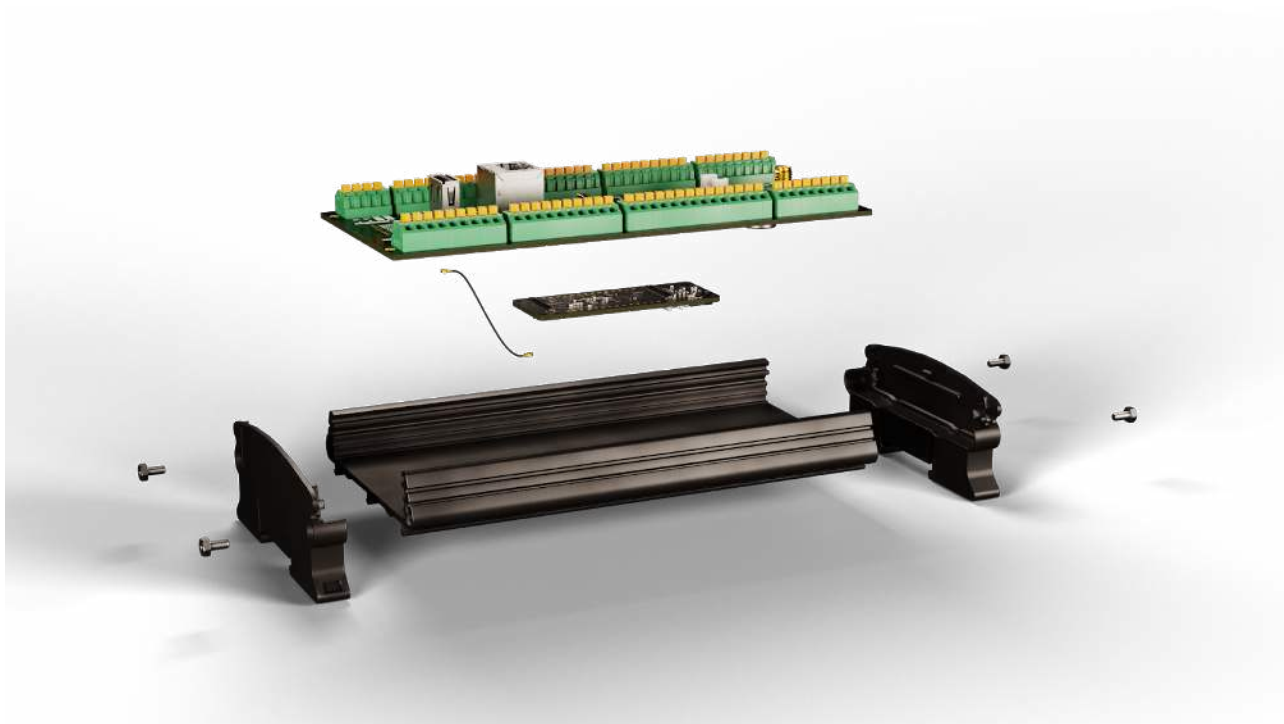
The Portenta Machine control exploded view
