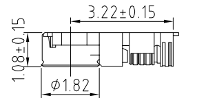
IPEX 4L PLUG DIMENSION
