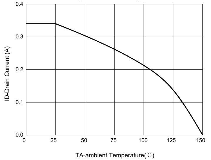
Fig. 10 - Current dissipation
