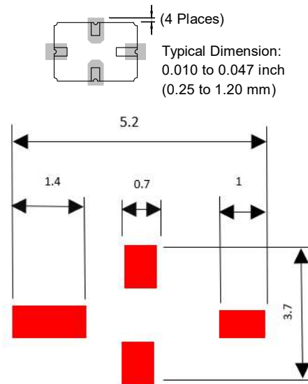
PCB Footprint
