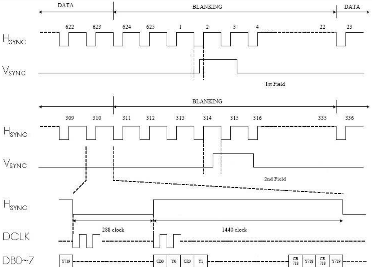
CCIR601 timing waveform (PAL)
